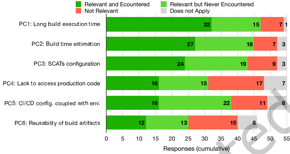
Fig. 4. Results of pipeline challenges perception: Pipeline Properties
