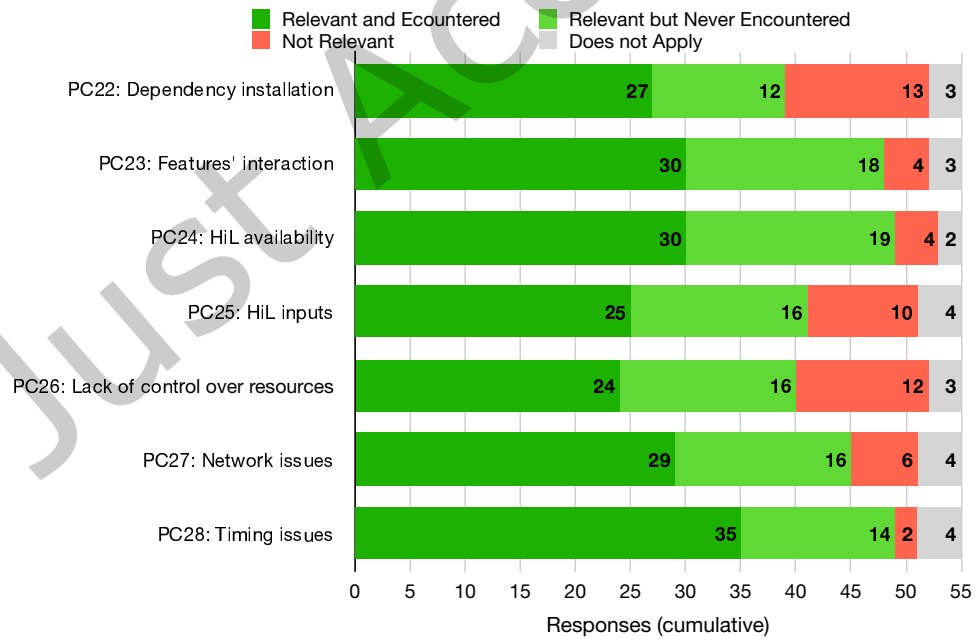
Fig. 8. Results of pipeline challenges perception: Flaky Behavior
