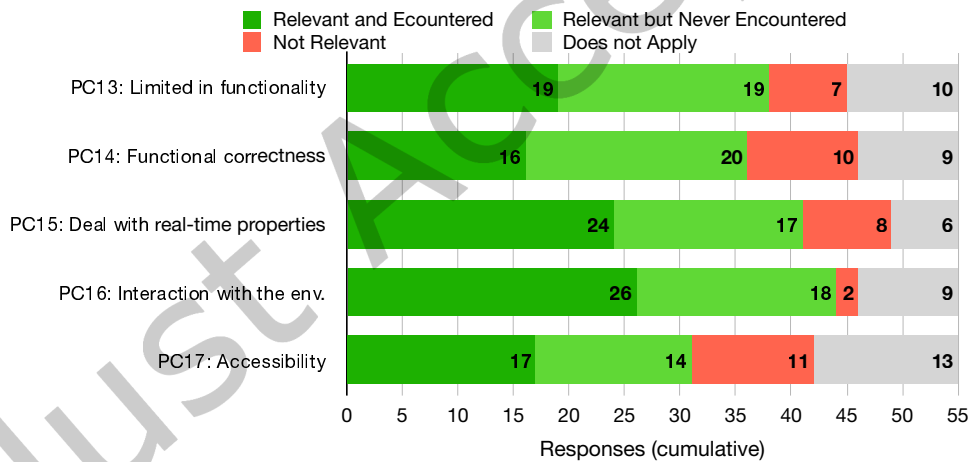
Fig. 6. Results of pipeline challenges perception: Simulators
