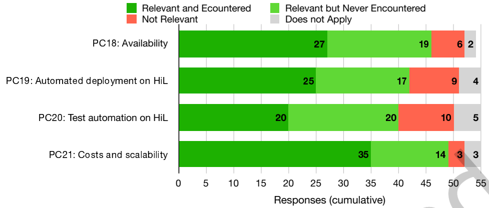
Fig. 7. Results of pipeline challenges perception: HiL
