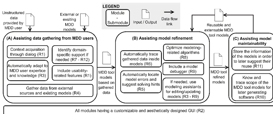
Fig. 5. Proposed emerging framework for modeling assistance in MDD tools.
