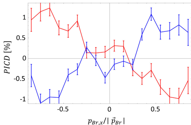
FIG. 1. Differential PICD as normalized difference between the enantiomers for CHBrClF as function of the angle between the bromine ion momentum and the direction of light propagation. The red curve reflects the measurement results for LCP, the blue for RCP. The error bars indicate the statistical error.
