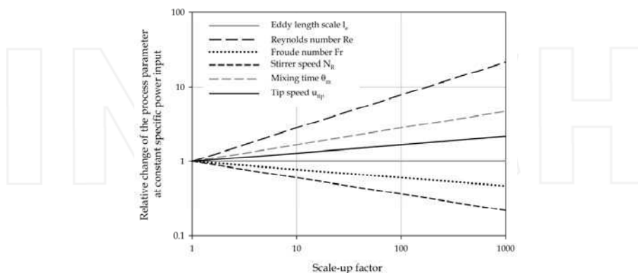
Fig. 1. Influence of scale on different process parameters at constant P/V
