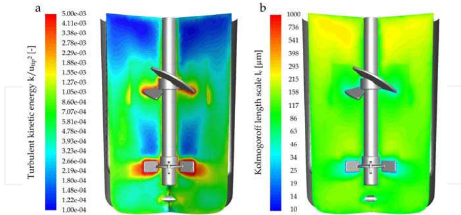
Fig. 11. Spatial distributions of the dimensionless turbulent kinetic energy k/u_{\text{tip}}^2 (a) and the Kolmogorov eddy size l_e (b) at P/V = 230 \text{ W}\cdot\text{m}^{-3} in the UniVessel® 2L single-use
