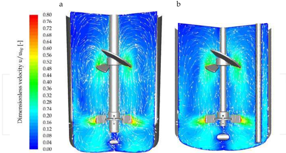
Fig. 3. Velocity distribution in the two small scale vessels UniVessel® single-use (a) and UniVessel® re-usable (b) represented by dimensionless velocity u/u_{tip} . The velocity magnitude is indicated by contour plots. The velocity vectors are projected to the given plains with fixed length
