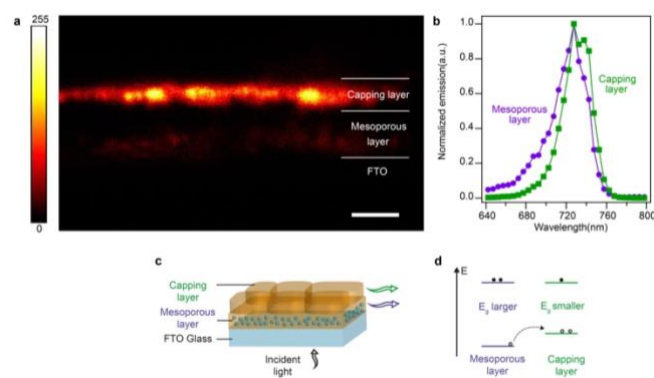
Figure 4. Study of the emission from the mesoporous layer and the capping layer in a partial cell. a) Cross-sectional CLSM imaging of CH 3 NH 3 PbI 3 sample consisting of a capping layer and the mesoporous perovskite infiltrated into an Al 2 O 3 mesoporous scaffold. Pseudo-color cross-sectional image of fully converted sample. 32 images showing the emission between 640 and 800 nm in steps of 5 nm each have been summed. Color scale assignment to the emission intensity in the image shown. Scale bar, 2.5 \mu m. b) Normalized emission from the perovskite in the capping layer and the mesoporous layer obtained from the images that make up 'a'. The emission from the mesoporous layer is blue-shifted compared to the capping layer. c) Schematic showing a view of a perovskite solar cell without a back contact. The emissions from the perovskite in the mesoporous layer and the capping layer in the partial cell are shown, d) energy band diagram depicting the perovskite levels in the mesoporous and capping layers.
