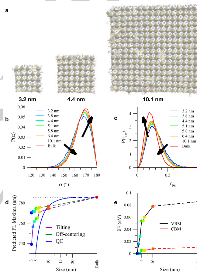
Figure 2. Results of atomistic simulations on \text{CH}_3\text{NH}_3\text{PbI}_3 nanocrystallites of increasing size. a ) Snapshots of the 3.2, 4.4 and 10.1 nm nanocrystallites taken from the classical MD. b ) Pb-I-Pb angular distribution function, P(\alpha) c ) Off-centering distribution, P(r_{\text{Pb}}) . The maximum of P(r_{\text{Pb}}) is at r_{\text{off}} \sim 0.2 nm, consistent with literature data on the \text{CsSnBr}_3 analogue [21] . d ) Estimated wavelength of the PL peak as a function of the nanocrystallite size due to Pb-I-Pb distortions, off-centering and quantum confinement. Theoretical values have been rigidly shifted to meet the bulk value. e ) Energy of the valence band maximum (VBM) and conduction band minimum (CBM) as a function of the nanocrystallite size due to Pb-I-Pb distortion. Data are relative to the smallest nanocrystallite, \Delta E = E(l) - E(3.2 \text{ nm}) . For reference, we also report data for an ideal (infinite) \text{CH}_3\text{NH}_3\text{PbI}_3 crystal. The colors of the symbols in 'd' and 'e' denote the sizes of the nanocrystallites according to the colors in the legend in 'b'. We remark that the difference between the band gap of a \sim 10 nm nanocrystallite and the bulk crystal due to surface-induced structural effects corresponds to a shift in emission of \sim 13 nm, while the difference due to QC is \sim 9 nm. We also look at the apparent abnormal trend of the predicted PL maximum of the 'tilting' curve (in 'd') and VBM curve (in 'e') between clusters of
