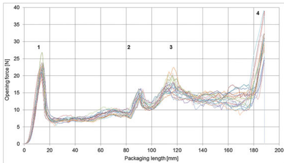
Figure 2. Opening force progression of thermoformed trays 'easy to open' with (1) the peel initiation force, (2) and (3) an increase of the opening force at the corners of the packaging and (4) the tearing-off force, which in this case equals the ultimate peel force.
