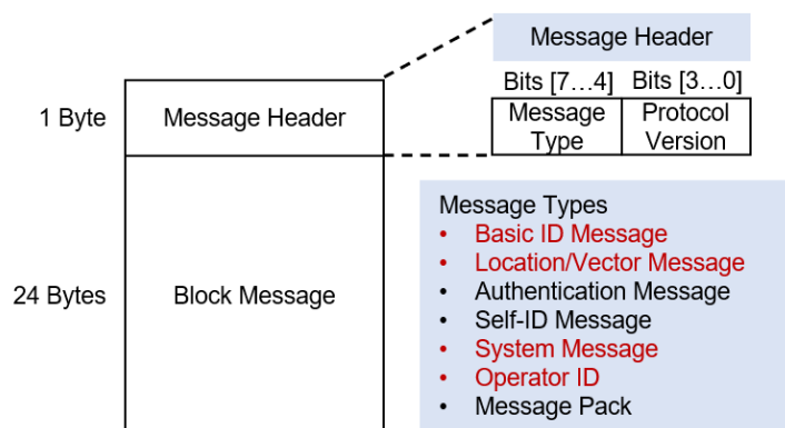
Figure 6: Message structure according to the ASTM and ASD-STAN standard
