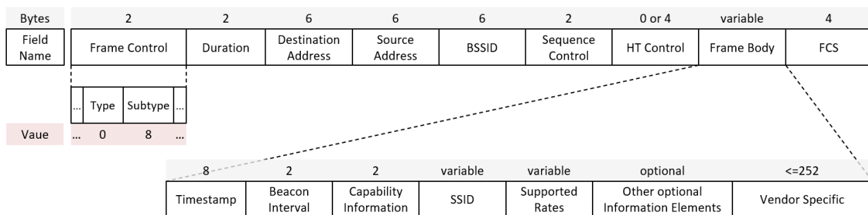
Figure 4: Structure of a Wi-Fi Beacon Frame including size in byte of each field (grey)
