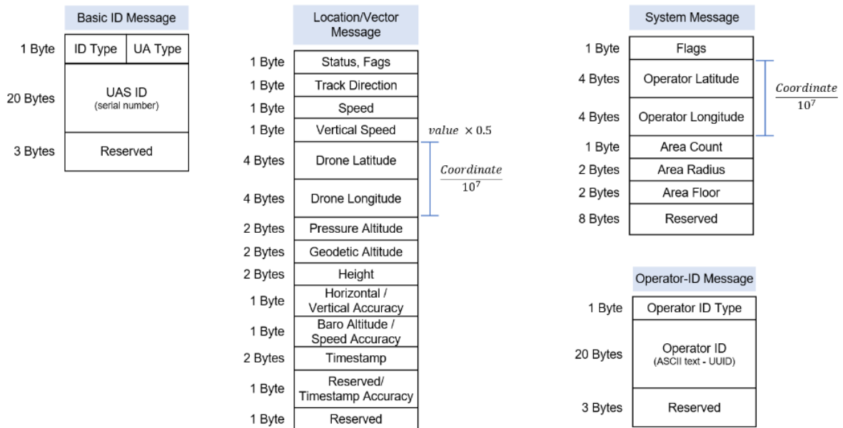
Figure 7: Structure of the four mandatory message types
